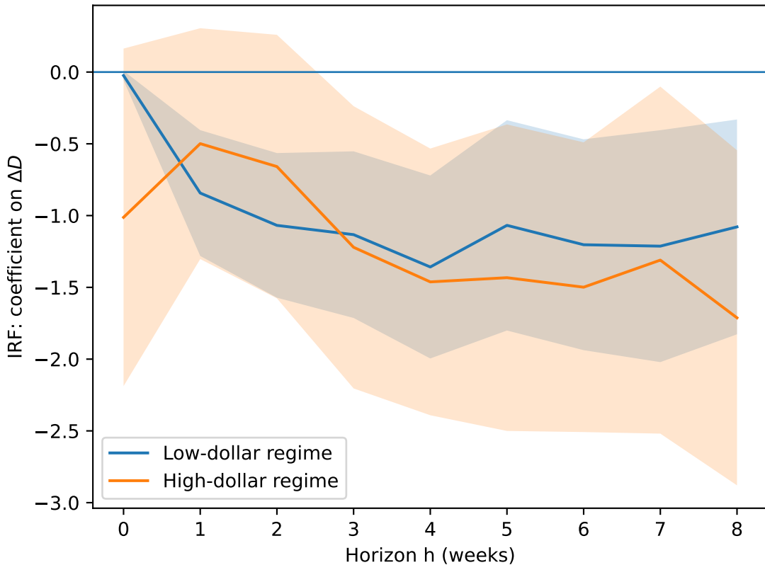
Regime-conditional local projections (JPY basis 20Y)
